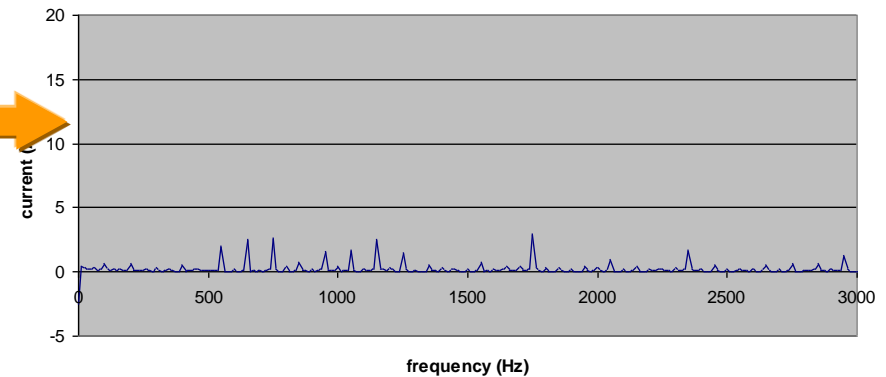
FFT neutral wire (with BLUEWAVE)
