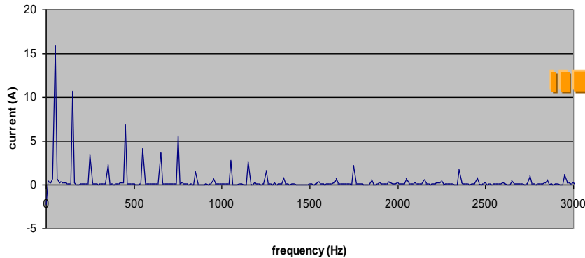
FFT neutral wire (without BLUEWAVE)
